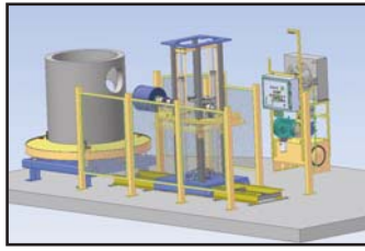
Auto Machine with Single Spindle and Standard Turntable (Uni-Directional Coring)
