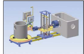
Auto Machine with Standard Turntable and Dual Opposed Spindles (Bi-Directional Coring)
