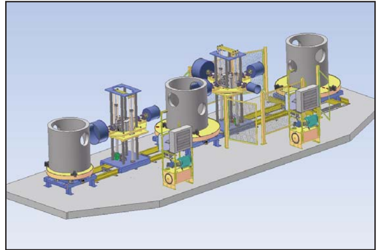
Multi-Coring Machine with TWO Auto Coring Units. ONE Offsetting Turntable and TWO Standard Turntables (Simultaneous Double Coring, Bi-Directional Coring, and Offset Hole Capability)
