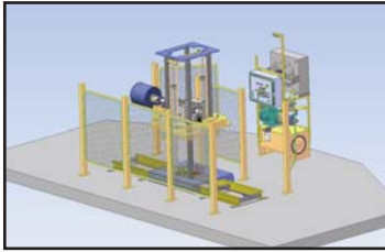
Basic Machine equipped with necessities for future upgrades (Uni-Directional Coring)
