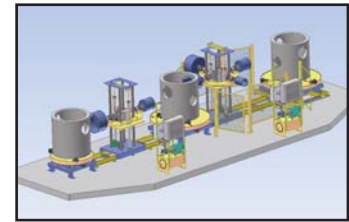
Multi-Coring Machine with TWO Auto Coring Units. ONE Offsetting Turntable and TWO Standard Turntables (Simultaneous Double Coring, Bi-Directional Coring, and Offset Hole Capability)
