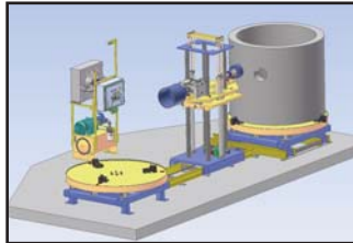
Auto Machine with One Offsetting Turntable and One Standard Turntable, and Dual Opposed Spindles (Bi-Directional Coring and Offset Hole Capability)
