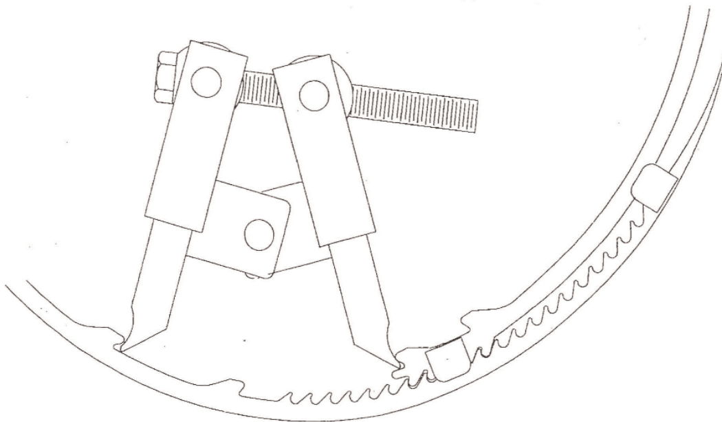
Tool & Sleeve as seen from Manhole Interior (preferred installation method)
