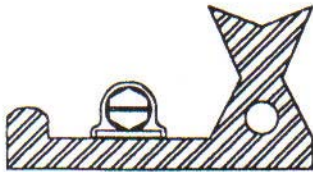
WS-30 WATERSTOP GASKET WITH TAKE-UP CLAMP
